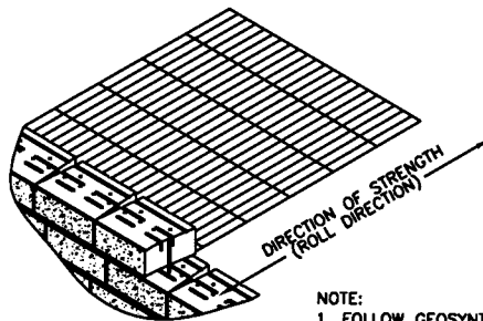
GEOSYNTHETIC INSTALLATION DETAIL SCALE: NONE
