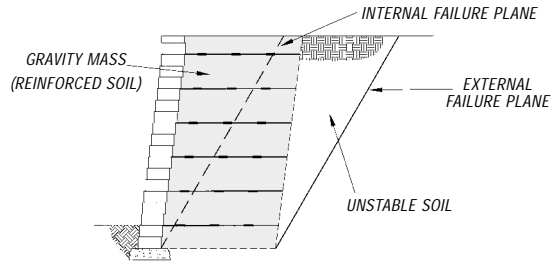
Reinforced Wall (Figure 1B)
