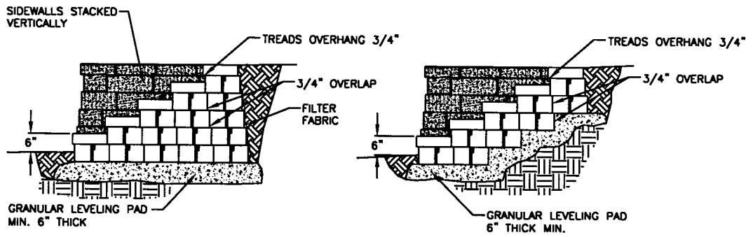
STAIR RISER DETAIL 1 BASE PEDESTAL METHOD (RECOMMENDED) SCALE: NONE
