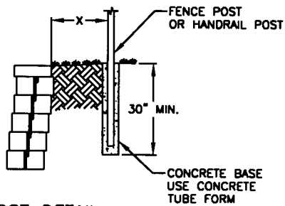
POST DETAIL TYPICAL HANDRAIL AND/OR FENCE POST SCALE: NONE
