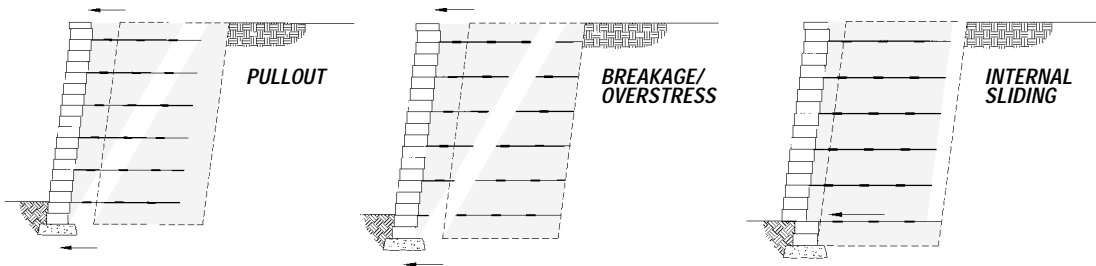
Internal Stability (Figure 2)
