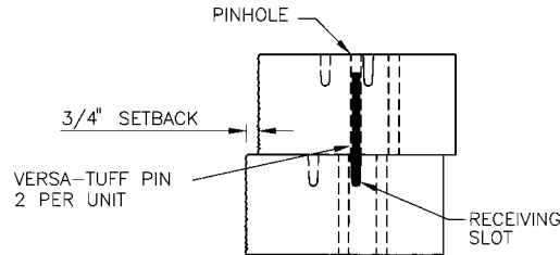
Pinning Detail
