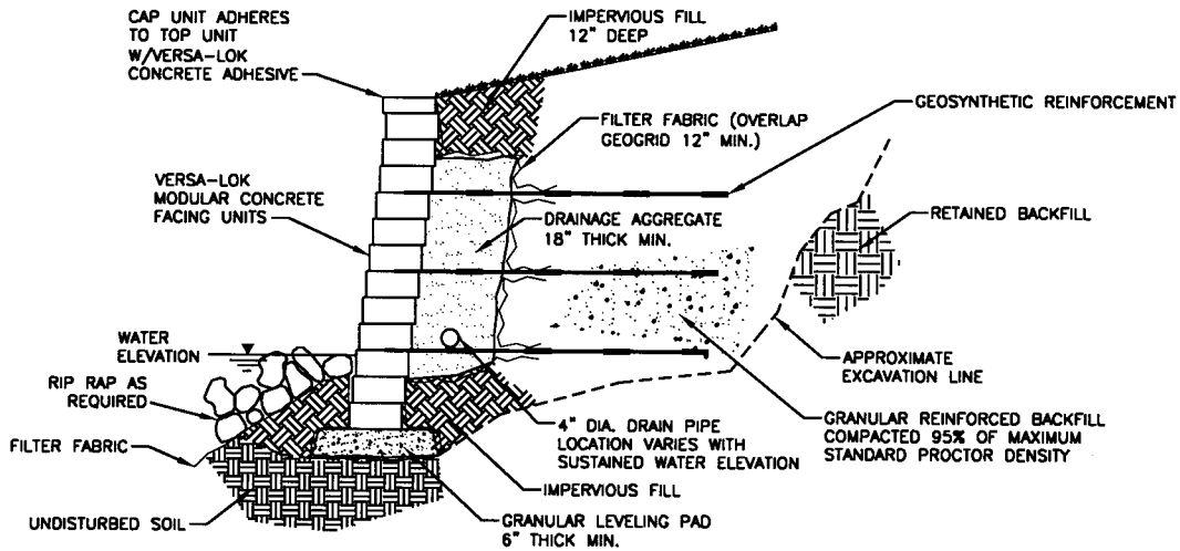
TYPICAL SECTION—REINFORCED SHORELINE WALL SCALE: NONE
