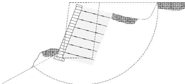
Global Stability (Figure 4)
