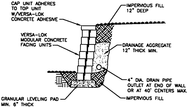
TYPICAL SECTION—UNREINFORCED RETAINING WALL SCALE: NONE
