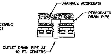
DRAIN DETAIL WALLS OVER 4' SCALE: NONE
