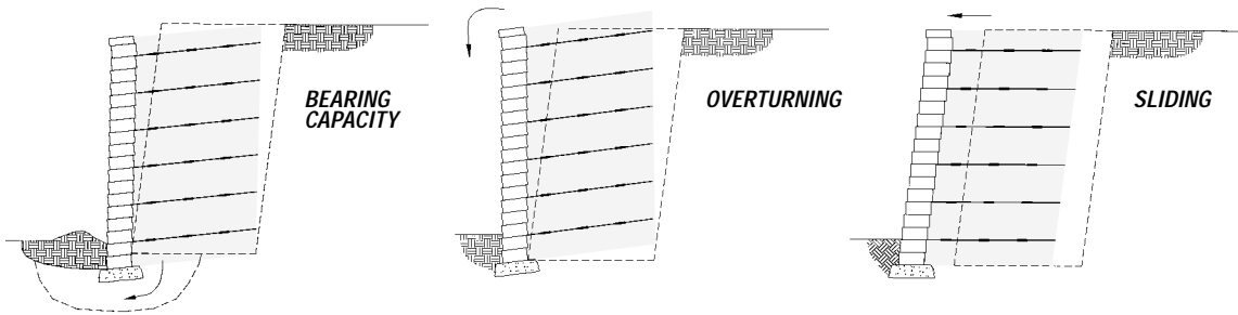
External Stability (Figure 3)
