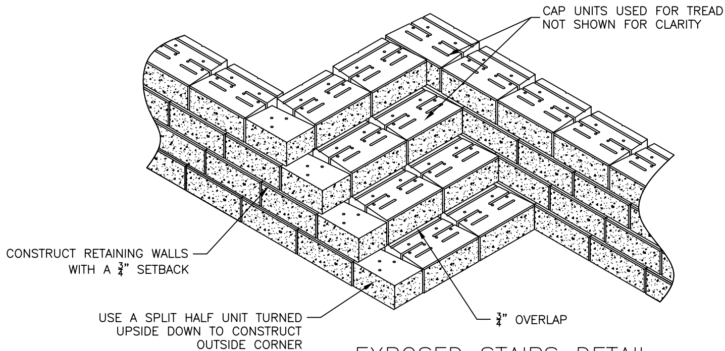
EXPOSED STAIRS DETAIL ONE SIDE EXPOSED STAIRS SCALE: NONE
